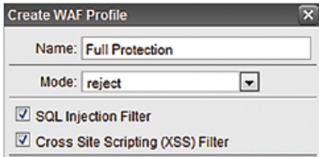
Firewall profile builder
